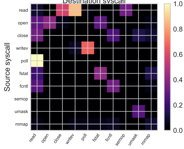
Destination syscall
