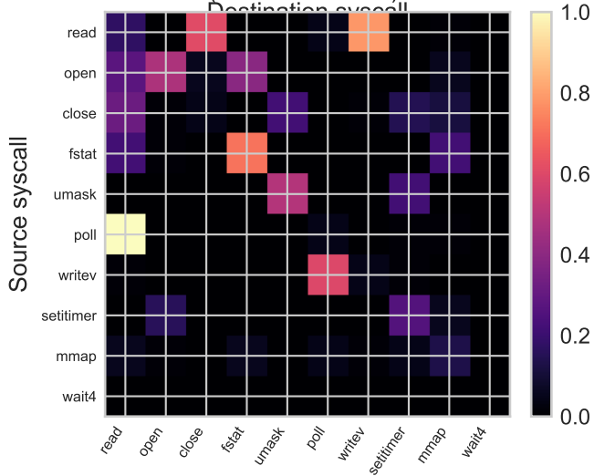
Destination syscall
